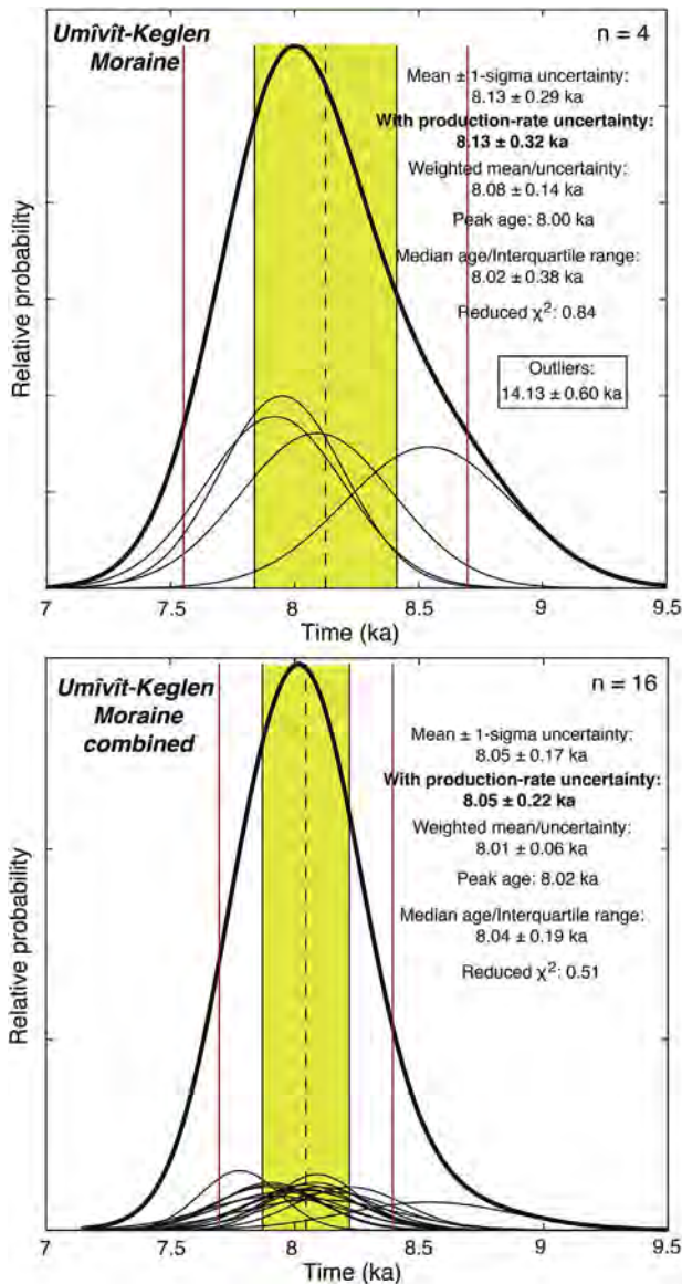
Fig. 16. Normal kernel density estimates for boulders on the Umivit-Keglen Moraine from this study (top panel), and for boulders on the Umivit-Keglen moraine from this study combined with Winsor et al. (2015) and Levy et al. (2018). We combine all three datasets to constrain the age of the Umivit-Keglen Moraine to 8.05 \pm 0.22 ka ( n = 16 ).
