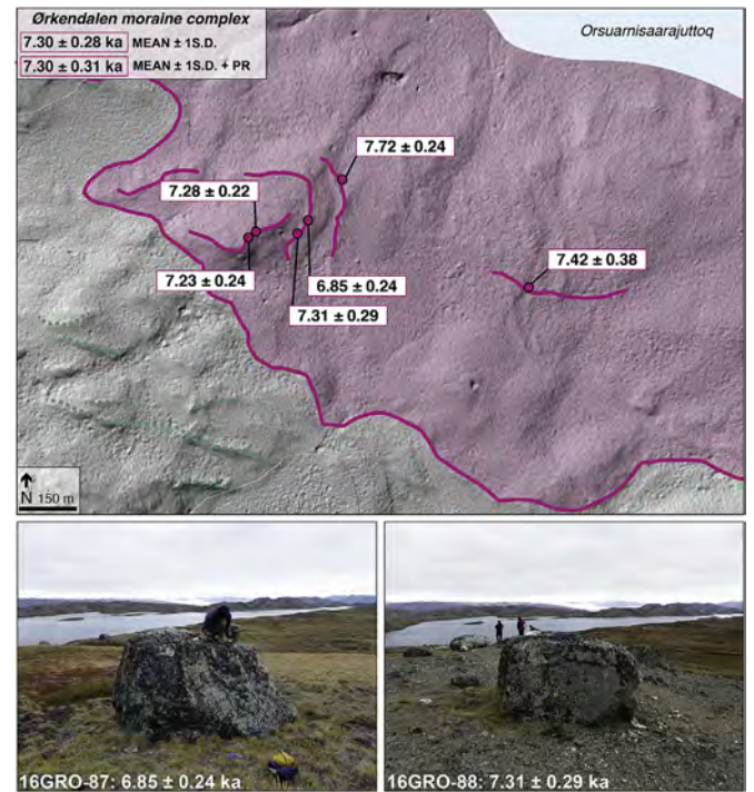
Fig. 14. Ørkendalen Moraine sample site with 10 Be ages and representative samples 16GRO-87 and 16GRO-88. These samples are from the outermost segment of Ørkendalen drift that is ~15 km from the modern ice margin. Located just beyond the Ørkendalen limit are minor recessional moraines (green dashed lines) that are part of the Umivît-Keglen Moraine system.
