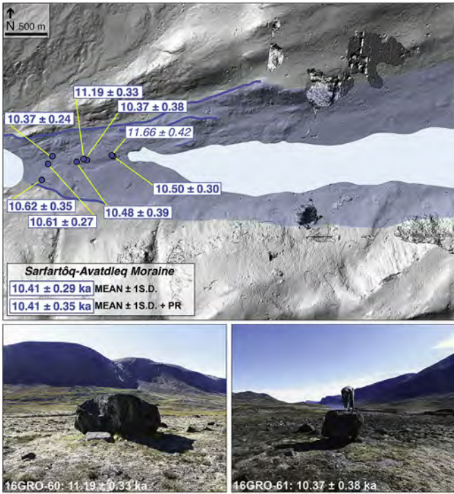
Fig. 11. Northern sampling site on the Sarfartøq-Avatdleq Moraine. Here the Sarfartøq-Avatdleq Moraine is mainly defined by a thin drift limit where patches of bedrock can be found among the drift. Shown are representative samples 16GRO-60 and 16GRO-61.
