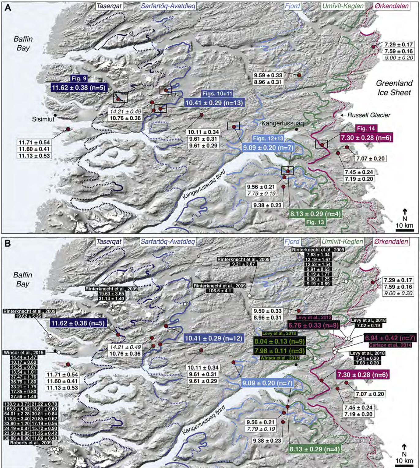
Fig. 3. (A) Moraines deposited by the GrIS between Baffin Bay and the modern ice margin during the early Holocene (Weidick, 1974; van Tatenhove et al., 1996). Shown are all individual 10 Be ages (ka ± 1SD analytical uncertainties) from erratic boulders perched on bedrock located beyond and between moraine systems (white boxes and black text; outliers in italics), and the arithmetic mean ± 1SD 10 Be age for each moraine (colored boxes and white text; Table 1; Fig. 15; Fig. 16). (B) Same as panel A, but includes all previously published 10 Be ages from region discussed in section 6.3 (Table S1).
